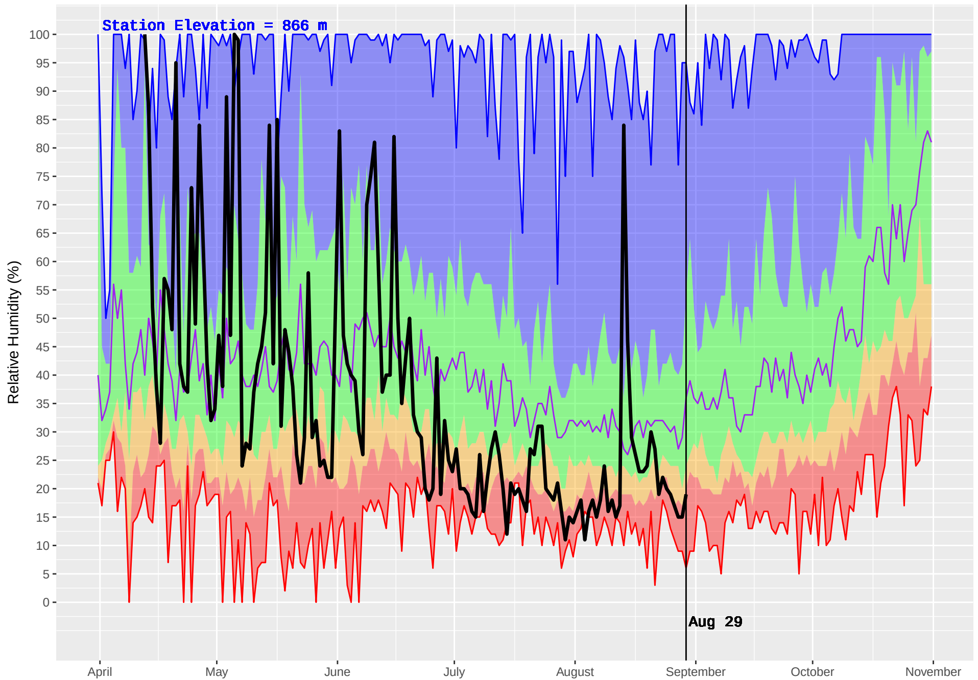
NICOLL (393) : Historical (1981–2016) and Current (2017) Noon Relative Humidity
