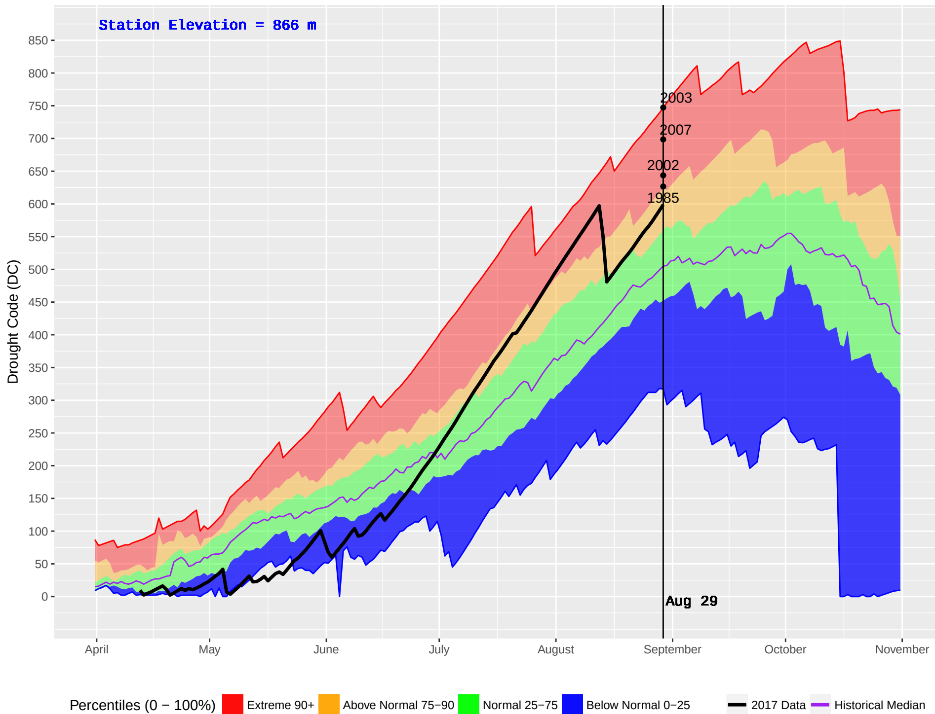
NICOLL (393) : Historical (1981–2016) and Current (2017) Noon Drought Code (DC)
