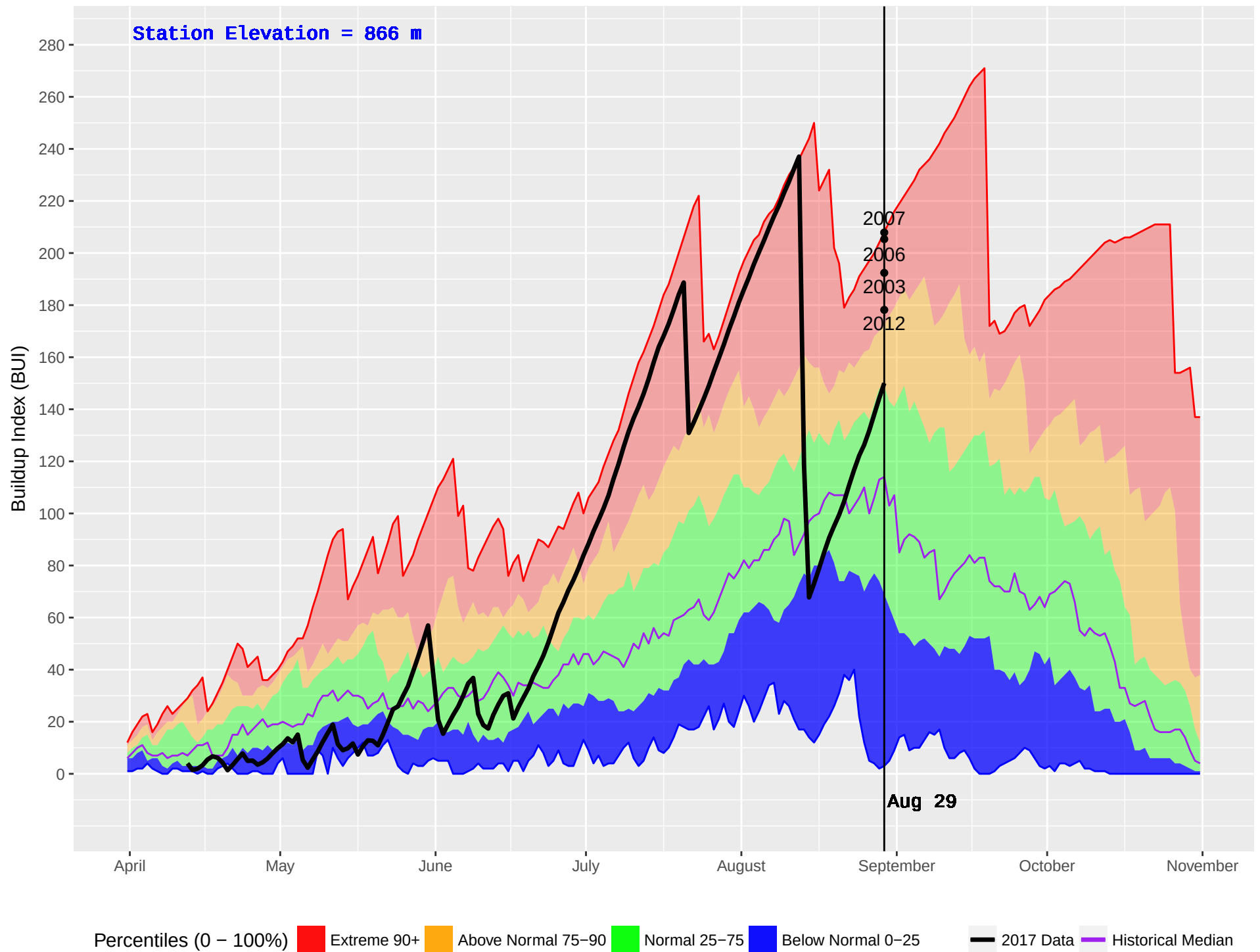
NICOLL (393) : Historical (1981–2016) and Current (2017) Noon Buildup Index (BUI)
