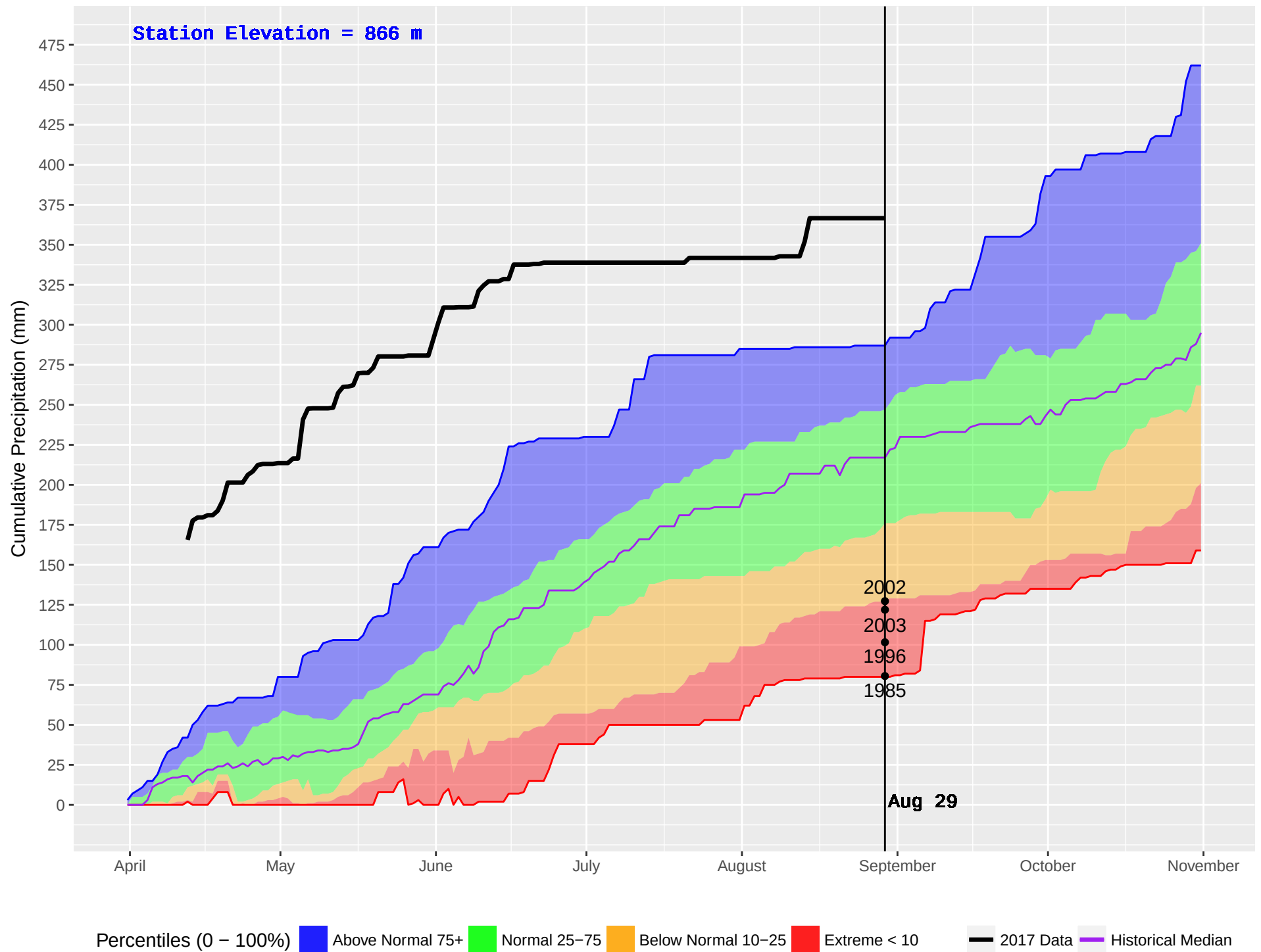
NICOLL (393) : Historical (1981–2016) and Current (2017) Noon Cumulative Precipitation
