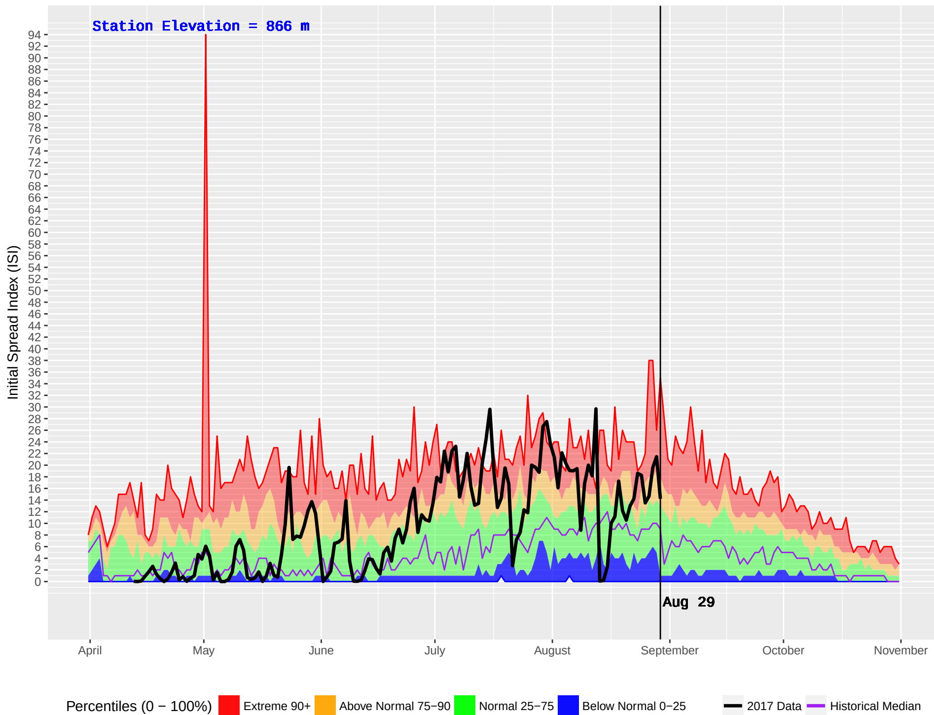
NICOLL (393) : Historical (1981–2016) and Current (2017) Noon Initial Spread Index (ISI)
