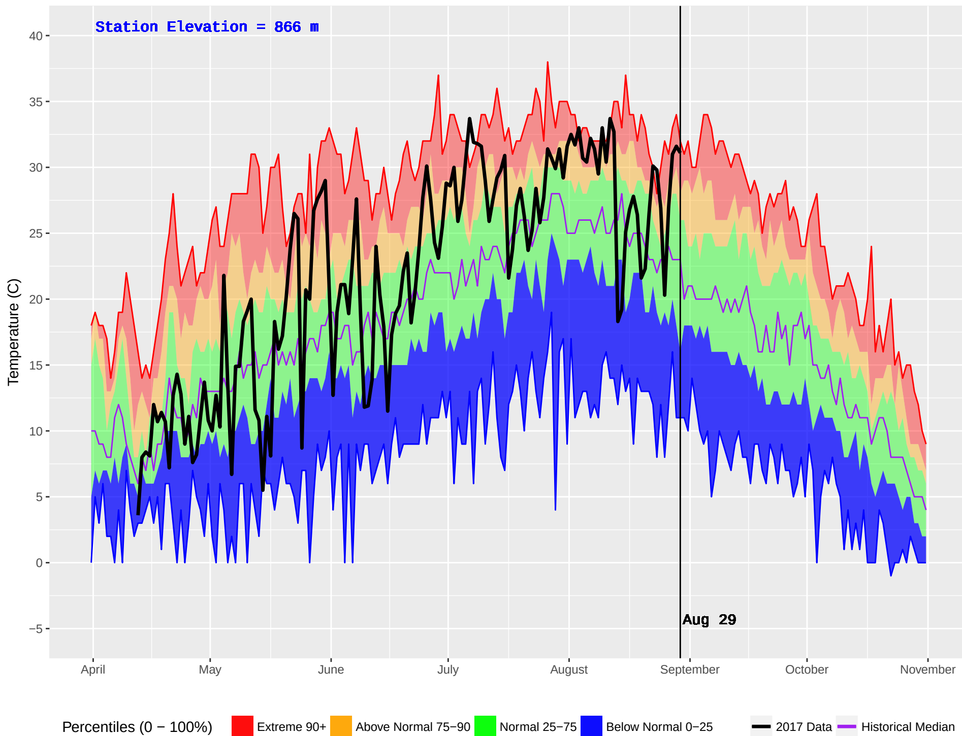
NICOLL (393) : Historical (1981–2016) and Current (2017) Noon Temperature
