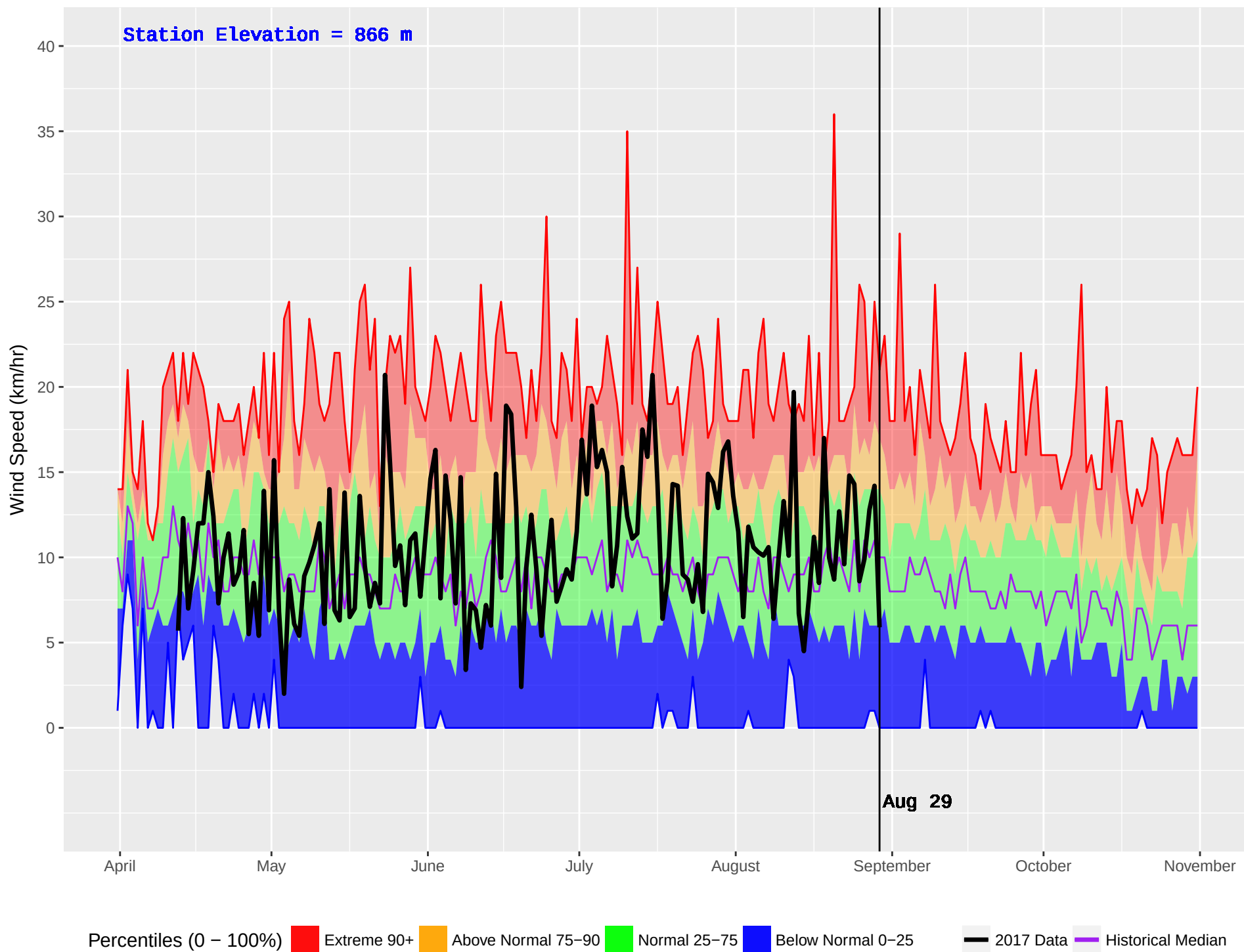
NICOLL (393) : Historical (1981–2016) and Current (2017) Noon Wind Speed
