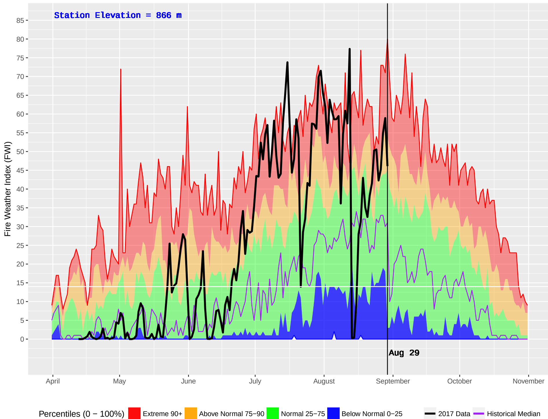
NICOLL (393) : Historical (1981–2016) and Current (2017) Noon Fire Weather Index (FWI)
